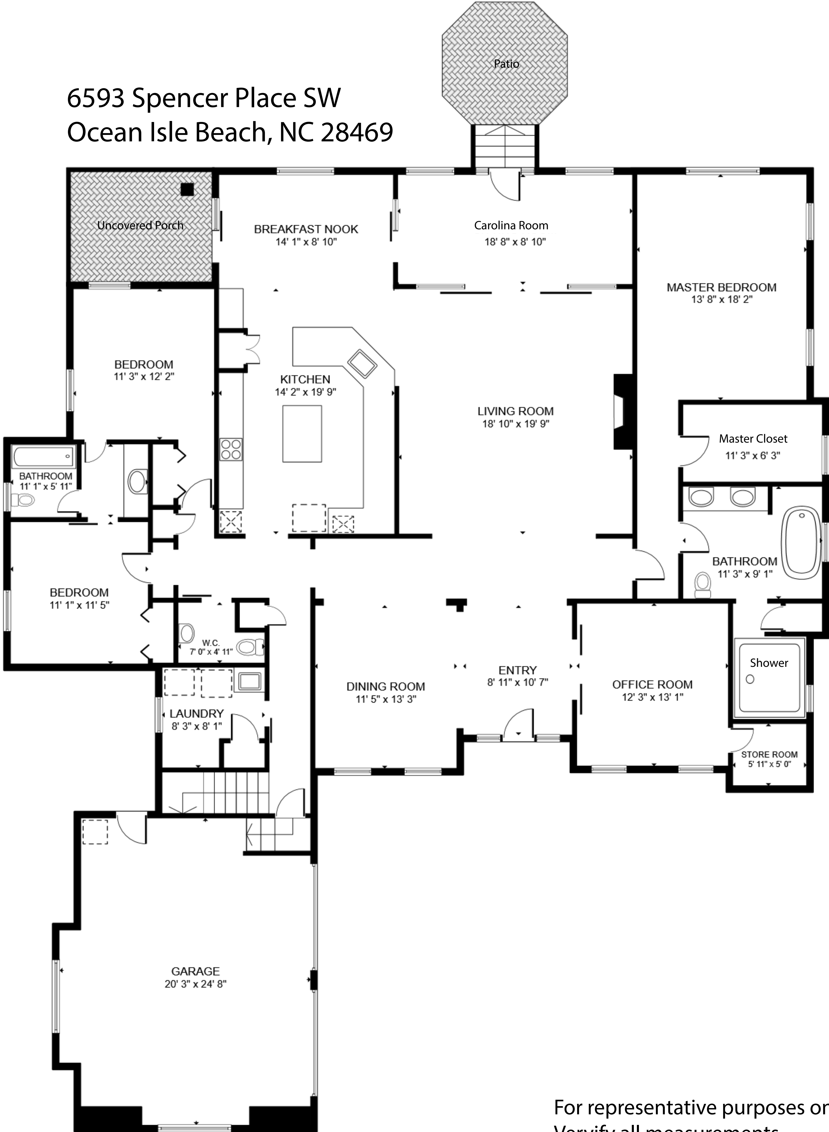
FLOOR 1
